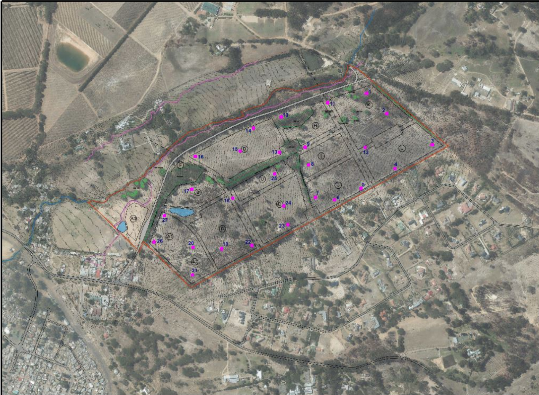
PLAN: TRIAL HOLE POSITIONS 1: 2500 (A1)
